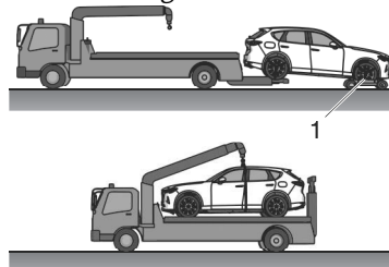
1. Wheel dollies
